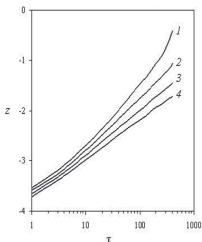
Fig. 2. Calculated dependences of the dust particle charge on temperature of electrons at various values of the degree of roughness of its surface: 0 (1) – smooth; 0,08 (2); 0,8 (3); (4) – smooth particle without accounting for emission
