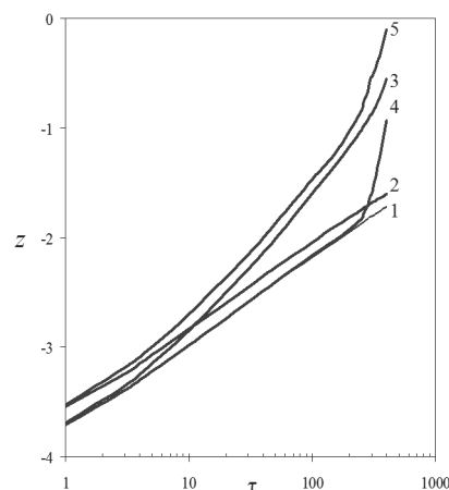
Fig. 3. Calculated dependences of the smooth dust particle charge on the temperature of electrons. (1) without accounting for emission; (2) taking into account ion – electronic and photoemissions; (3) taking into account secondary emission of electrons; 4 – only thermoemission is considered; 5 – all types of emission are considered
